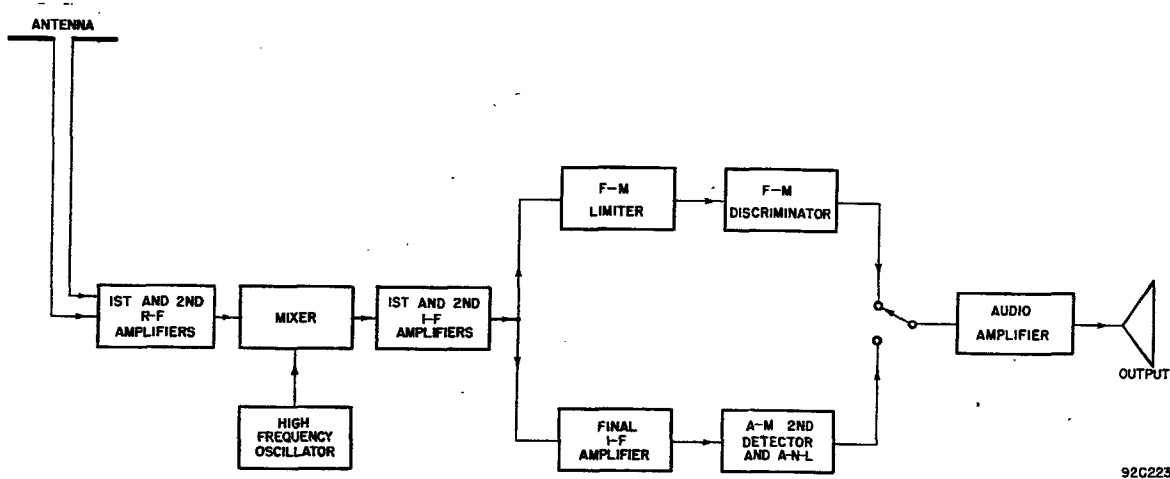
Fig. 4-1. Radio Receiver Model S-37, block diagram
